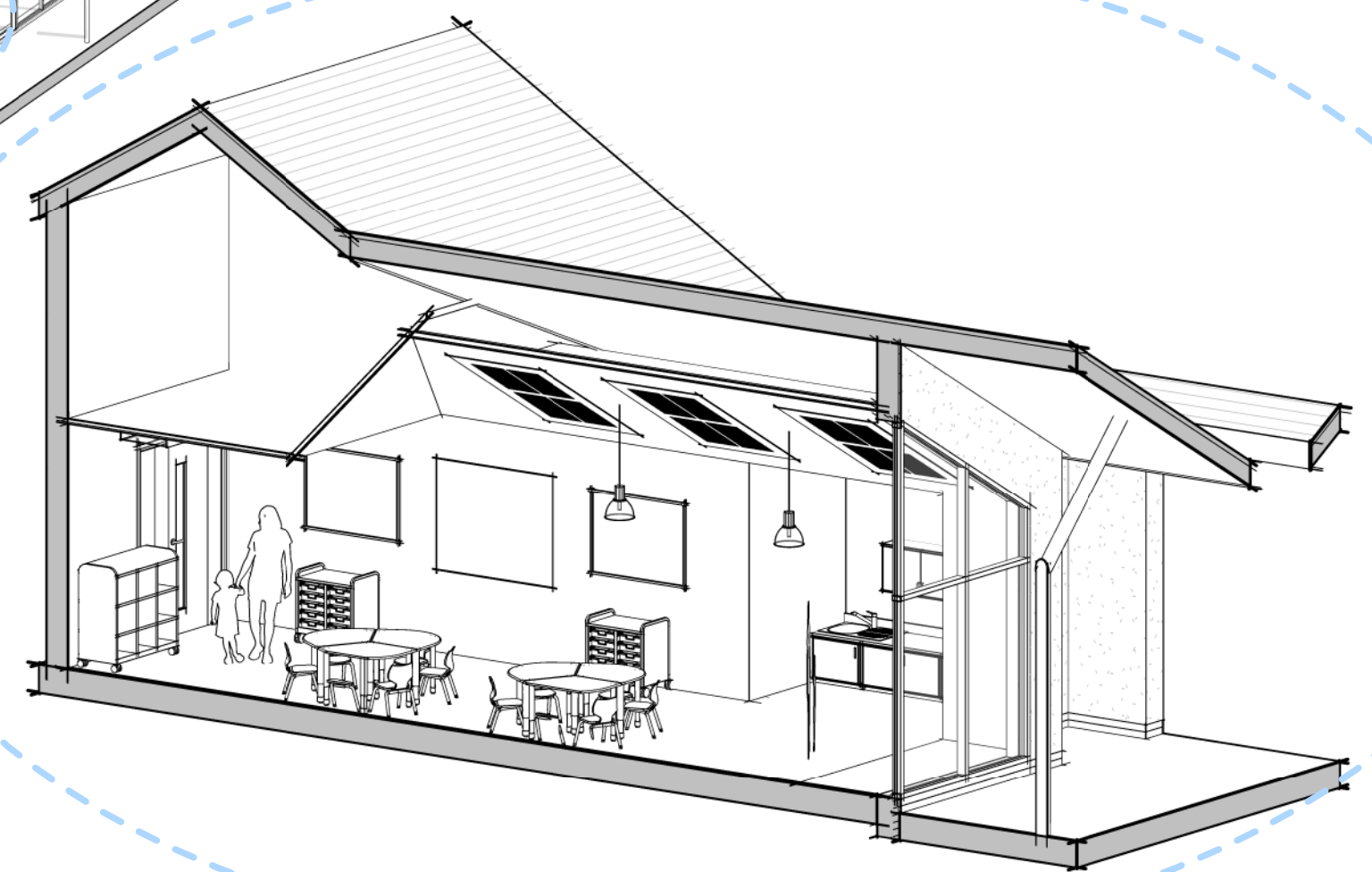
TRAWSDORIAD DOSBARTH BABANOD
